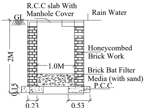
Details Of Rain Water Collection Pit (Recharge Well Method) SCALE:- (NTS)
