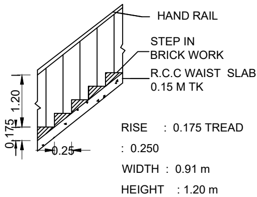
STAIR DETAILS
