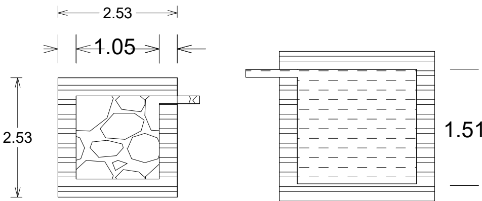
RWH_CAPACITY_L=1000LTRS DETAILS OF FILTER BED & WELL
