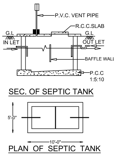
PLAN OF SEPTIC TANK
