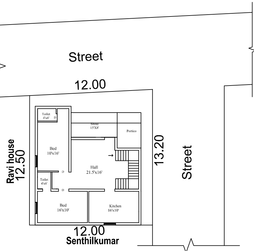
SITE PLAN
