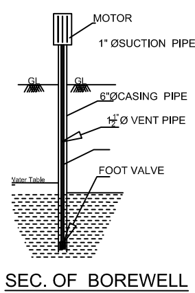
SEC. OF BOREWELL
