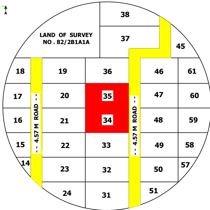
TOPO PLAN ( SCALE 1: 2000 )
