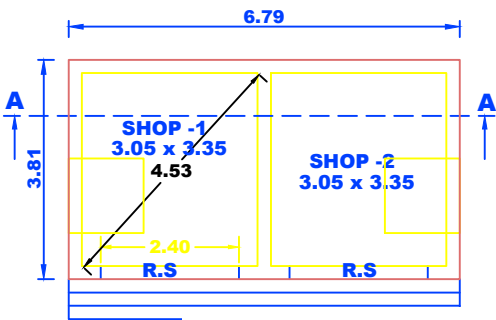
PLAN
