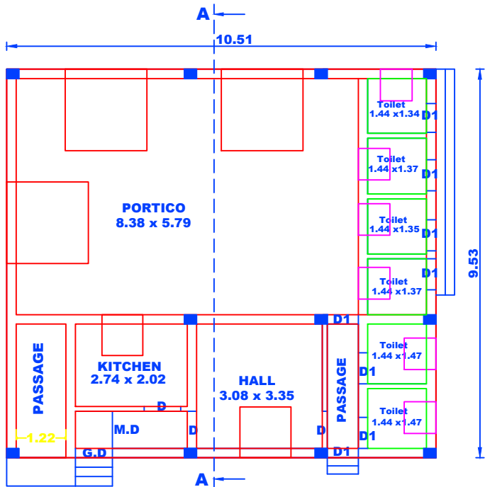
PLAN BLOCK-2
