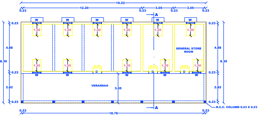
PLAN(BLOCK-1)
