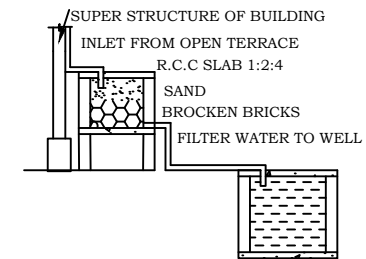
RAINWATER HARVESTING
