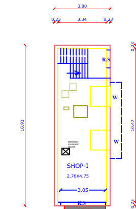
SHOP-I PROPOSED GROUND FLOOR PLAN
