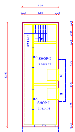
SHOP-I SHOP-II PROPOSED FIRST FLOOR PLAN
