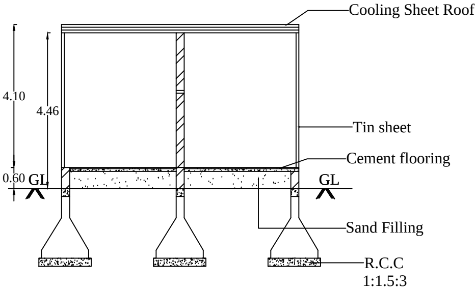
CROSS SECTION"AB"
