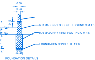
FOUNDATION DETAILS
