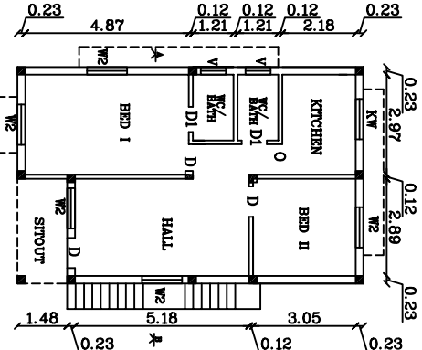
GROUND FLOOR PLAN 1
