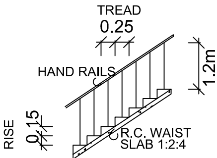
STAIRCASE DETAILS
