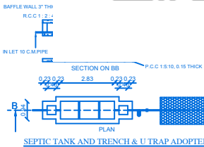
SEPTIC TANK AND TRENCH & U TRAP ADOPTED
