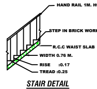
STAIR DETAIL
