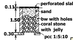
percolation pit
