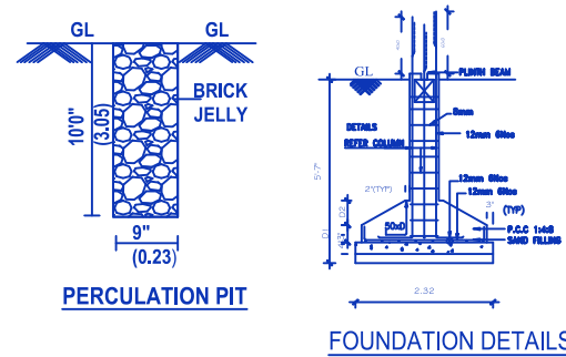
FOUNDATION DETAILS
