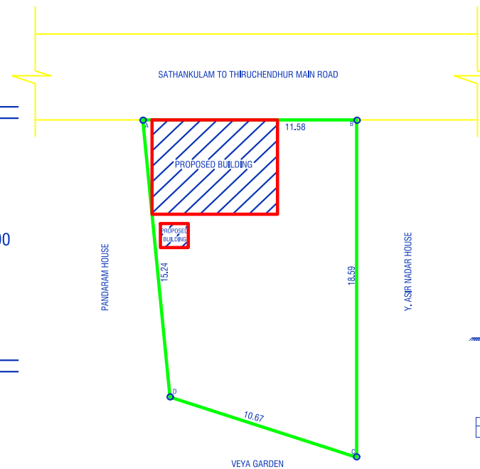
SITE PLAN
