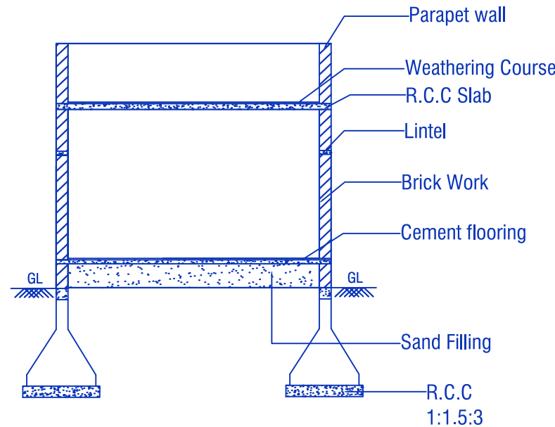
CROSS SECTION ON AB'
