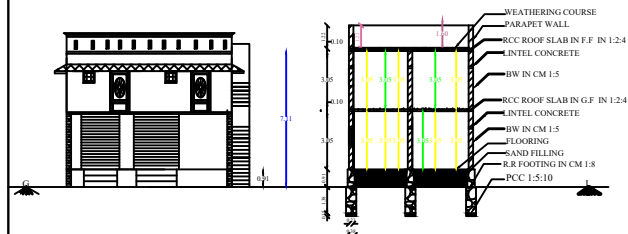
SECTION ON AB&CD
