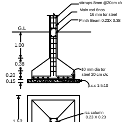
Details of COLUMN
