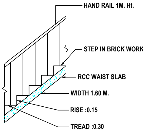
STAIR DETAIL
