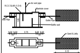
SEPTIC TANK & TRENCH
