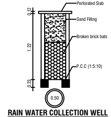
RAIN WATER COLLECTION WELL
