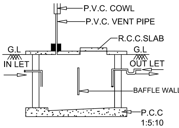
SEC. OF SEPTIC TANK
