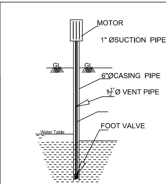
SEC. OF BOREWELL
