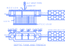
SEPTIC TANK AND TRENCH
