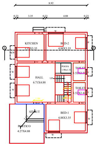
G.FLOOR PLAN
