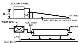
Details of solar water heating system
