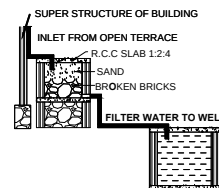
RAINWATER HARVESTING
