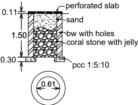
percolation pit
