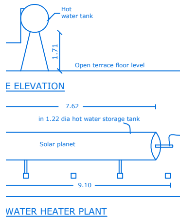
WATER HEATER PLANT
