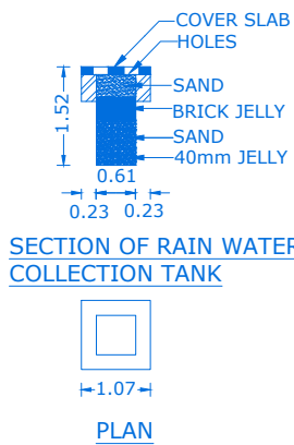
SECTION OF RAIN WATER COLLECTION TANK PLAN
