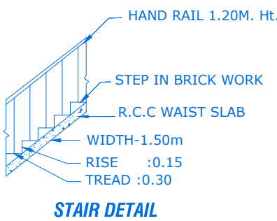
STAIR DETAIL
