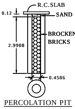
PERCOLATION PIT
