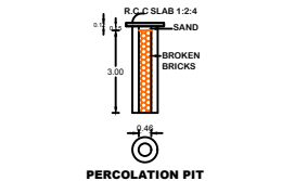
PERCOLATION PIT
