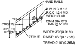
STAIRCASE DETAILS
