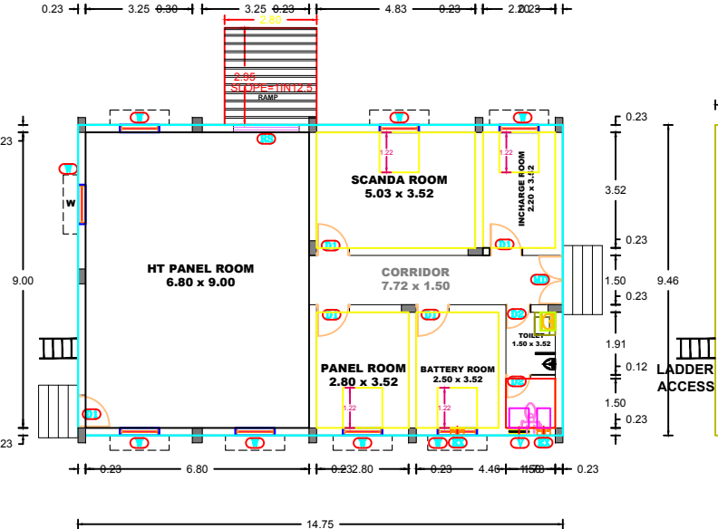
GROUND FLOOR PLAN FOR THE PROPOSED BUILDING
