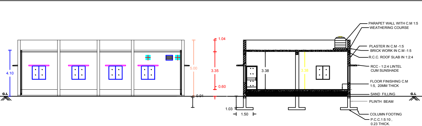
FRONT ELEVATION FOR THE PROPOSED BUILDING
