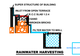
RAINWATER HARVESTING
