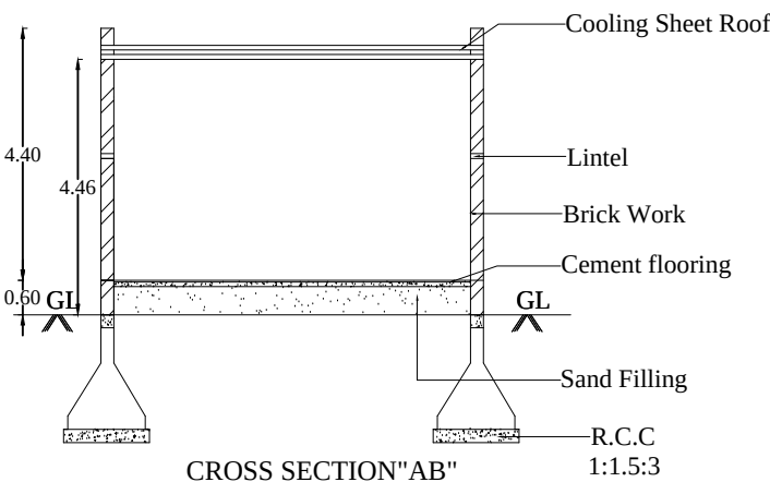
CROSS SECTION"AB"
