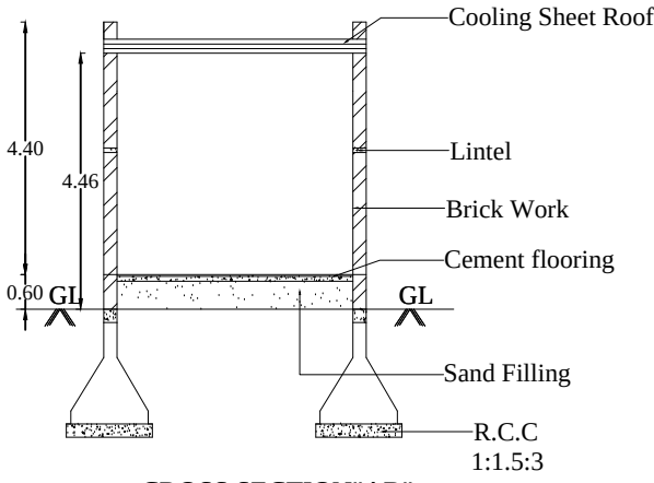
CROSS SECTION"AB"
