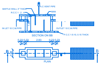
SEPTIC TANK AND TRENCH & UTRAP ADOPTED.
