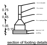
section of footing details
