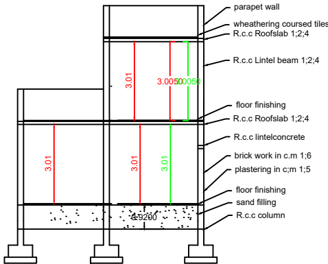
SECTION ON XX MURUGASAN EXG HOUSE
