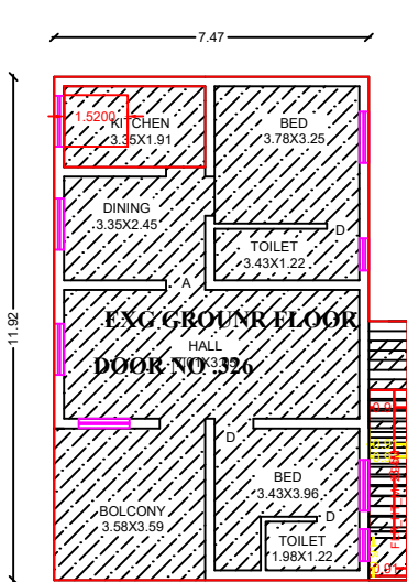
GROUND EXG FLOOR PLAN
