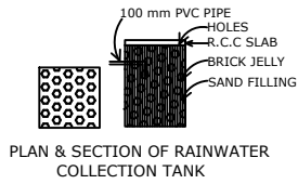
PLAN & SECTION OF RAINWATER COLLECTION TANK
