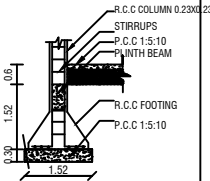
COLOUMN DETAILS
