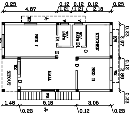
GROUND FLOOR PLAN 1
