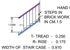
DETAILS OF STAIRCASE
