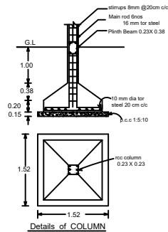
Details of COLUMN
