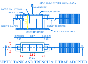
SEPTIC TANK AND TRENCH & U TRAP ADOPTED
