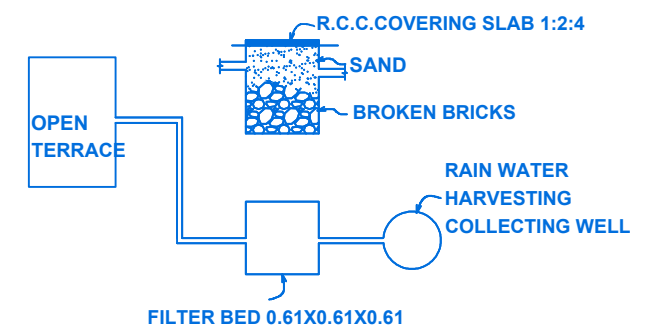
DETAILS OF RAIN WATER HARVESTING SYSTEM
