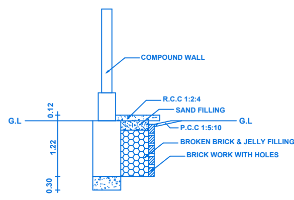
PLINTH BOUNDARY PERCOLATION PIT
