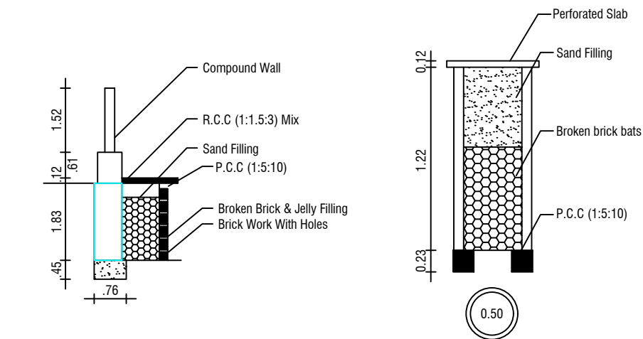
RAIN WATER HARVEST DETAILS
