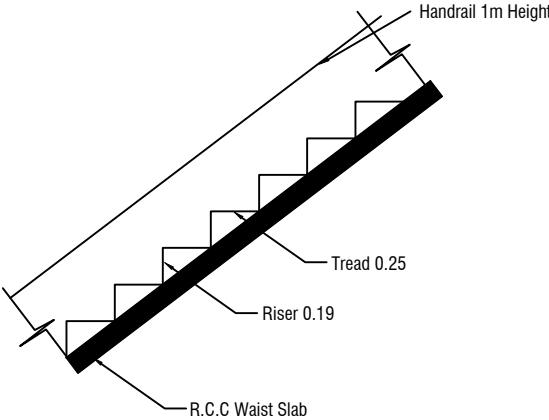
STAIR DETAILS
