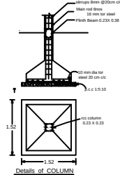
Details of COLUMN
