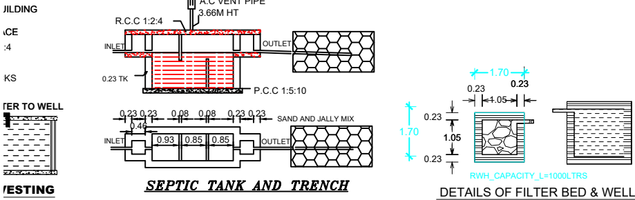
DETAILS OF FILTER BED & WELL
