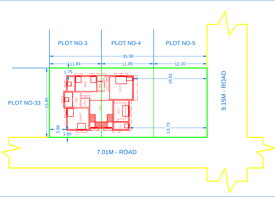
LOCATION PLAN Scale 1:400
