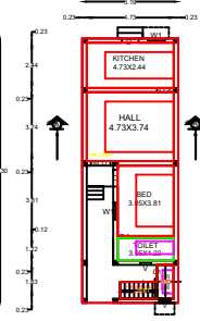
PRO.GROUND FLOOR PLAN
