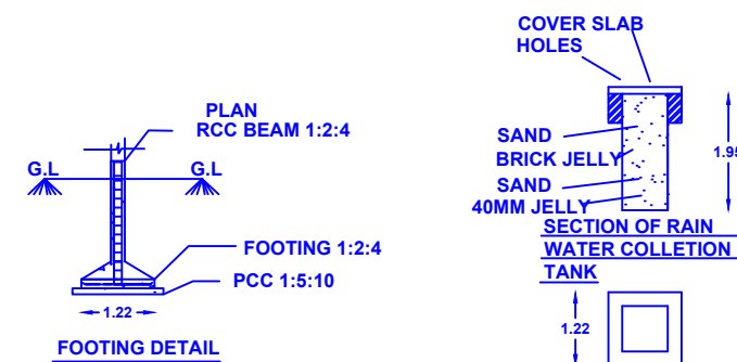
FOOTING DETAIL
