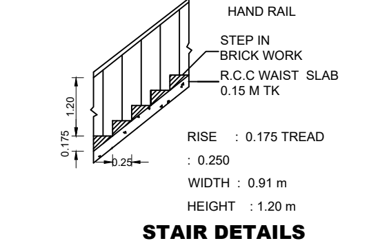
STAIR DETAILS
