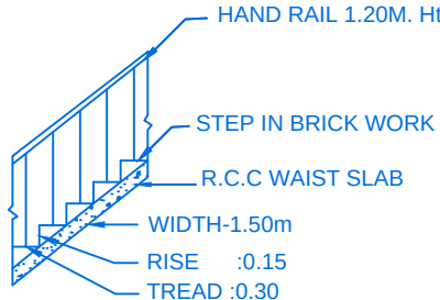
STAIR DETAIL
