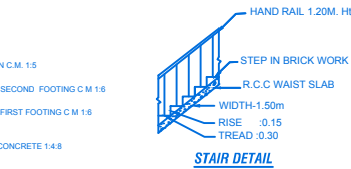
STAIR DETAIL
