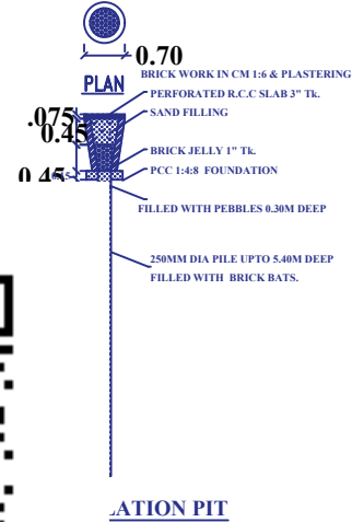
RAINWATER HARVESTING
