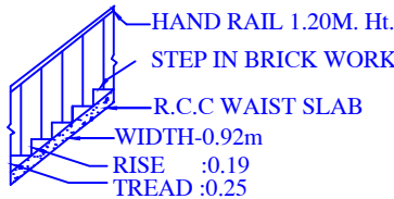
STAIR DETAIL
