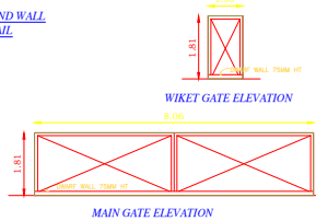
MAIN GATE ELEVATION
