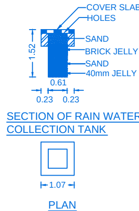
SECTION OF RAIN WATER COLLECTION TANK
