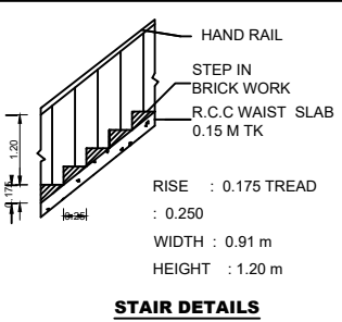
STAIR DETAILS
