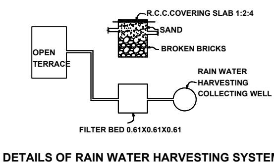
DETAILS OF RAIN WATER HARVESTING SYSTEM
