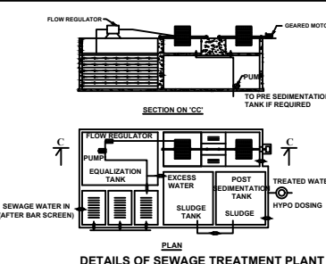
DETAILS OF SEWAGE TREATMENT PLANT
