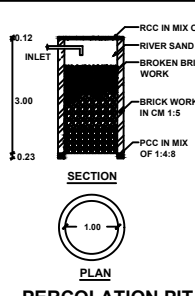
PERCOLATION PIT
