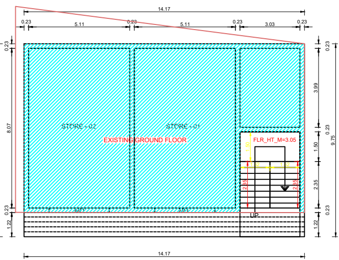
EXS.GROUND FLOOR PLAN
